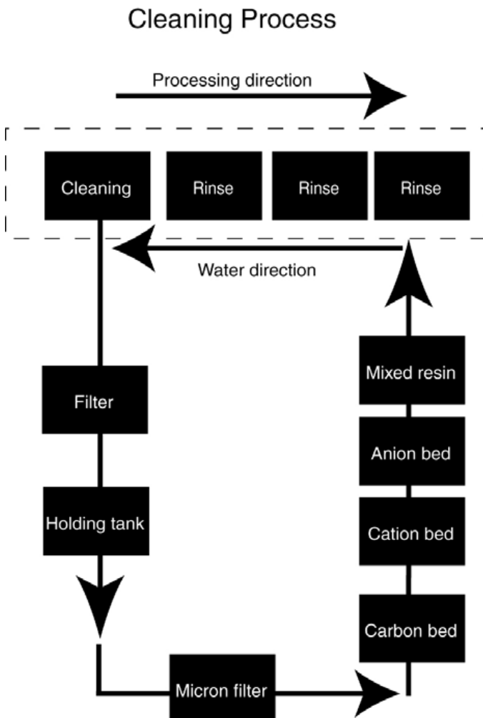
Figure 1. In-Line cleaning cycle
